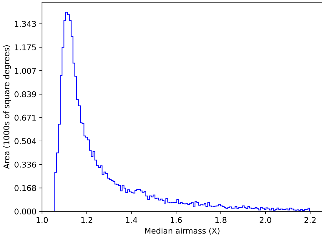
too_elab_r64_d3_ugrizy_v3.4_10yrs Yr 1 z band: Median airmass
