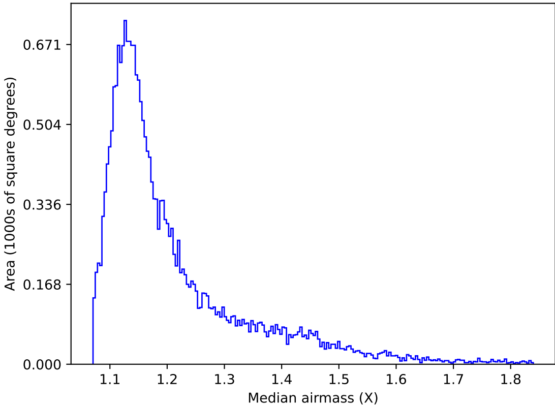
too_elab_r64_d3_ugrizy_v3.4_10yrs Yr 1 y band: Median airmass
