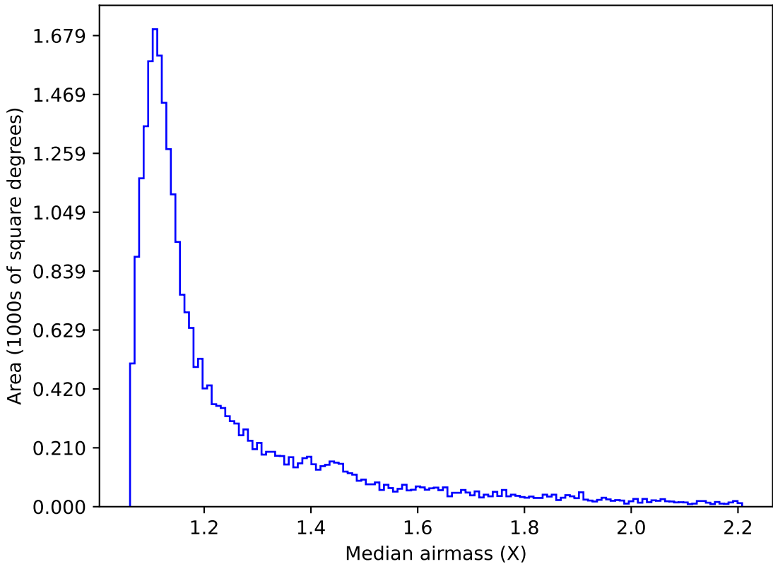
too_elab_r64_d3_ugrizy_v3.4_10yrs Yr 1 i band: Median airmass
