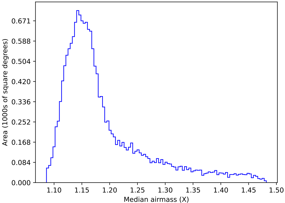
too_elab_r64_d3_ugrizy_v3.4_10yrs WFD z band: Median airmass
