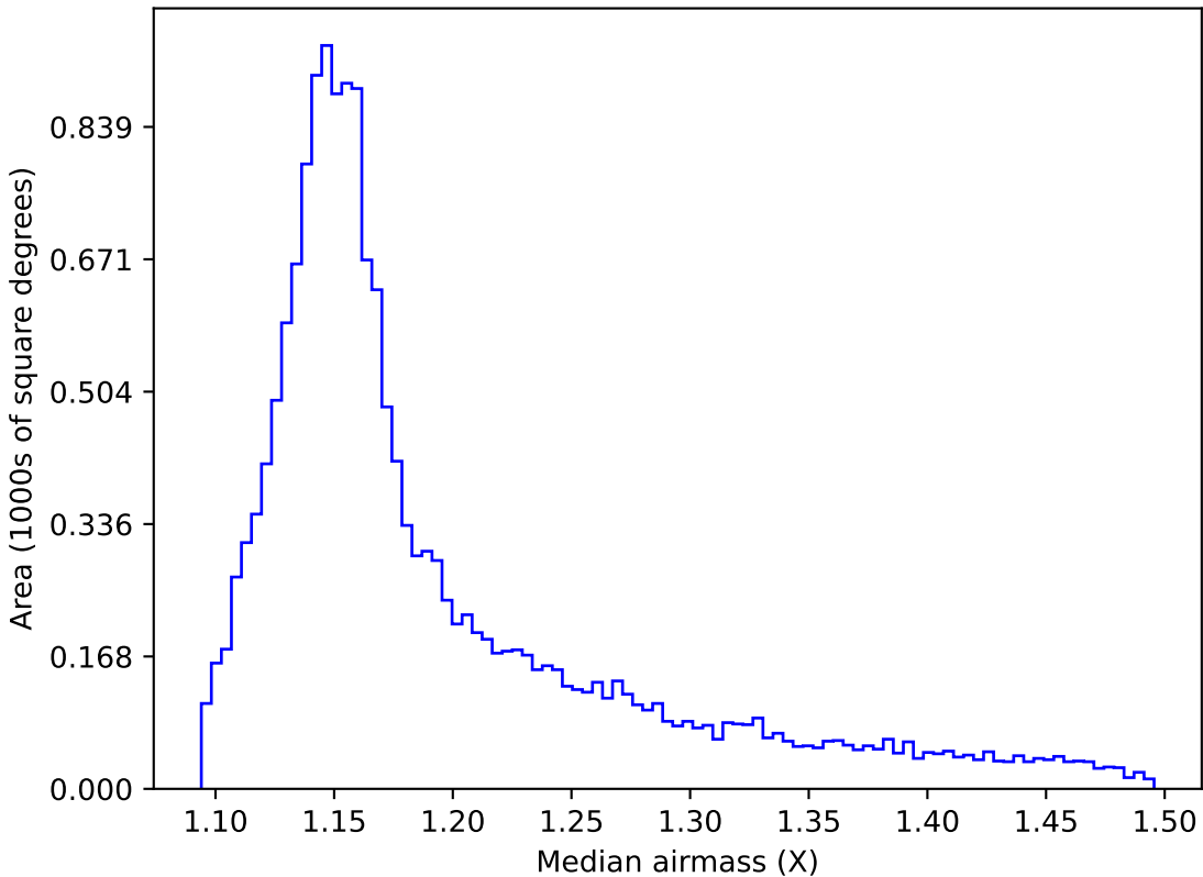
too_elab_r64_d3_ugrizy_v3.4_10yrs WFD y band: Median airmass
