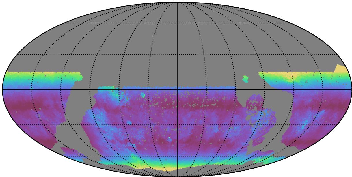
too_elab_r64_d3_ugrizy_v3.4_10yrs WFD u band: Median airmass
