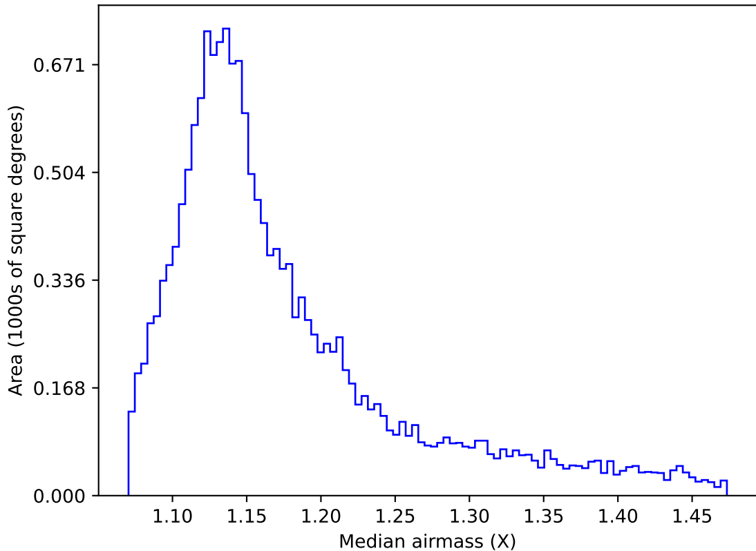
too_elab_r64_d3_ugrizy_v3.4_10yrs WFD u band: Median airmass
