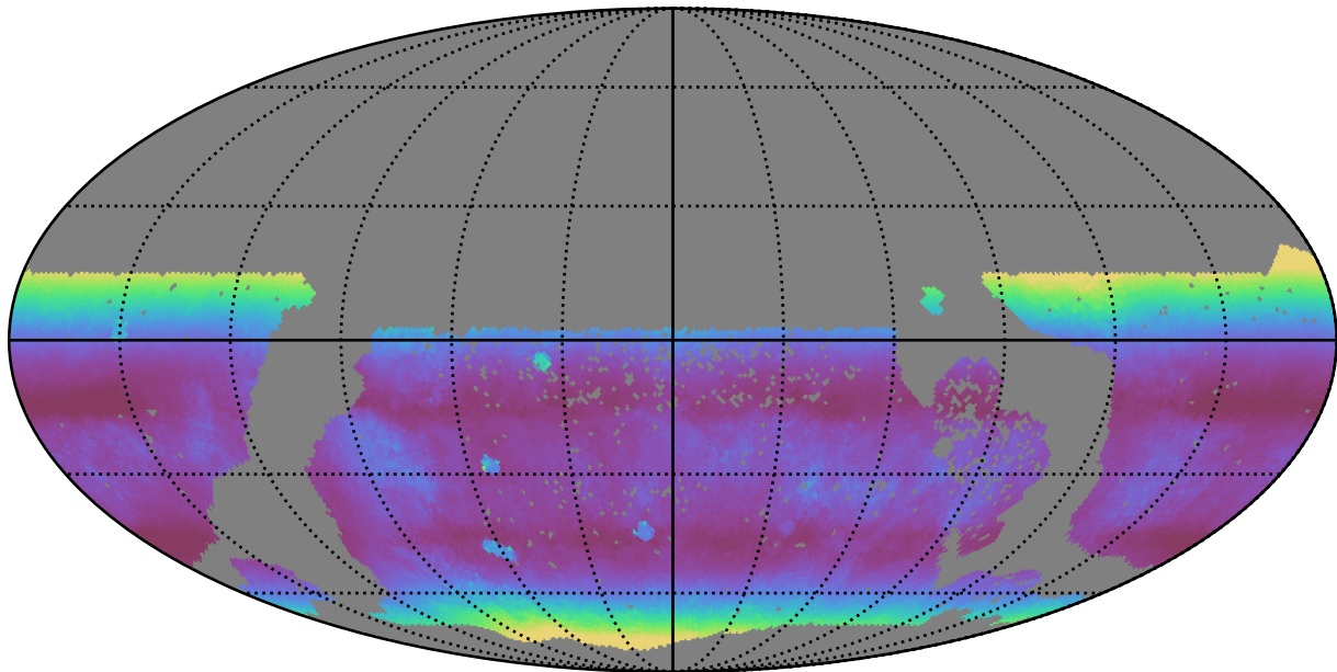
too_elab_r64_d3_ugrizy_v3.4_10yrs WFD r band: Median airmass
