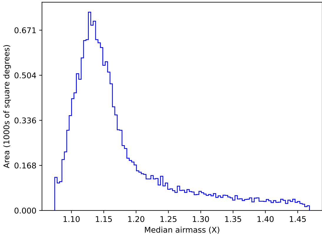
too_elab_r64_d3_ugrizy_v3.4_10yrs WFD r band: Median airmass
