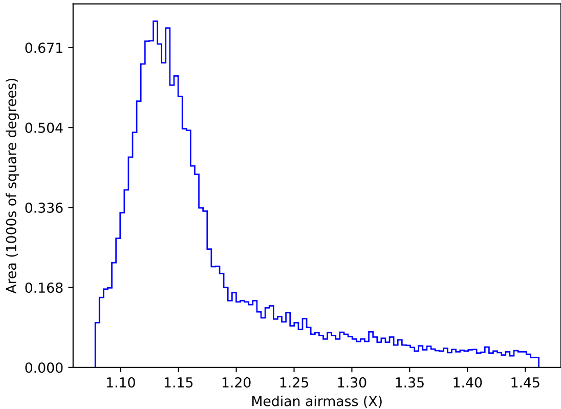
too_elab_r64_d3_ugrizy_v3.4_10yrs WFD i band: Median airmass
