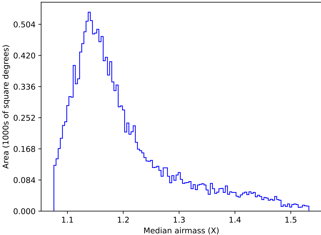
too_elab_r64_d3_ugrizy_v3.4_10yrs WFD g band: Median airmass
