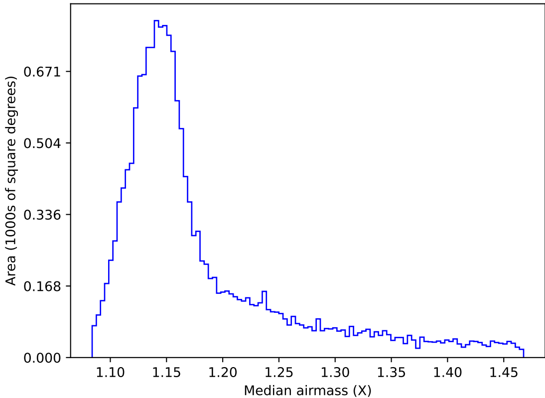
too_elab_r64_d3_ugrizy_v3.4_10yrs WFD all bands: Median airmass
