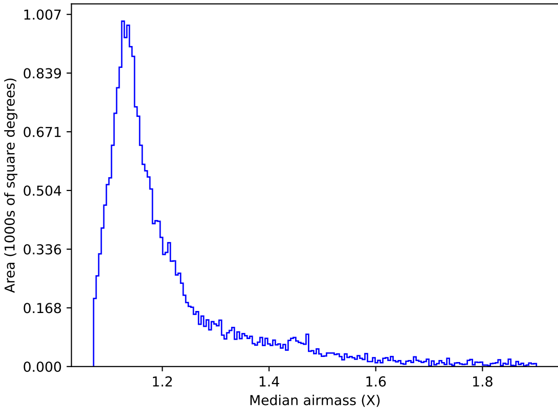
too_elab_r64_d3_ugrizy_v3.4_10yrs All sky u band: Median airmass
