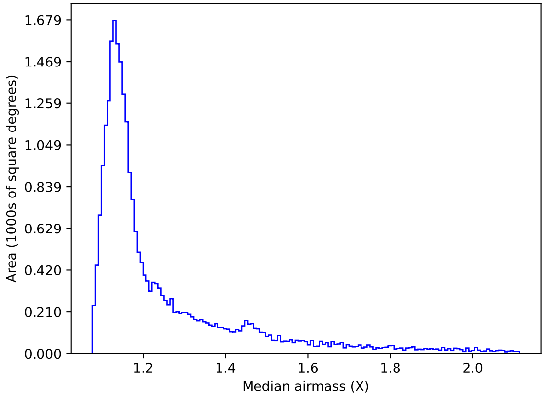
too_elab_r64_d3_ugrizy_v3.4_10yrs All sky r band: Median airmass
