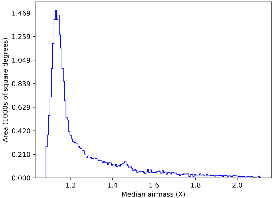
too_elab_r64_d3_ugrizy_v3.4_10yrs All sky i band: Median airmass
