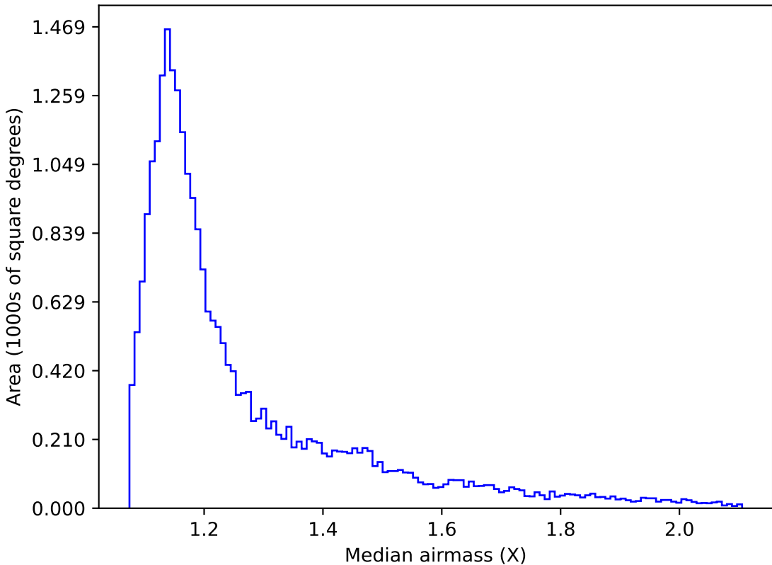
too_elab_r64_d3_ugrizy_v3.4_10yrs All sky g band: Median airmass
