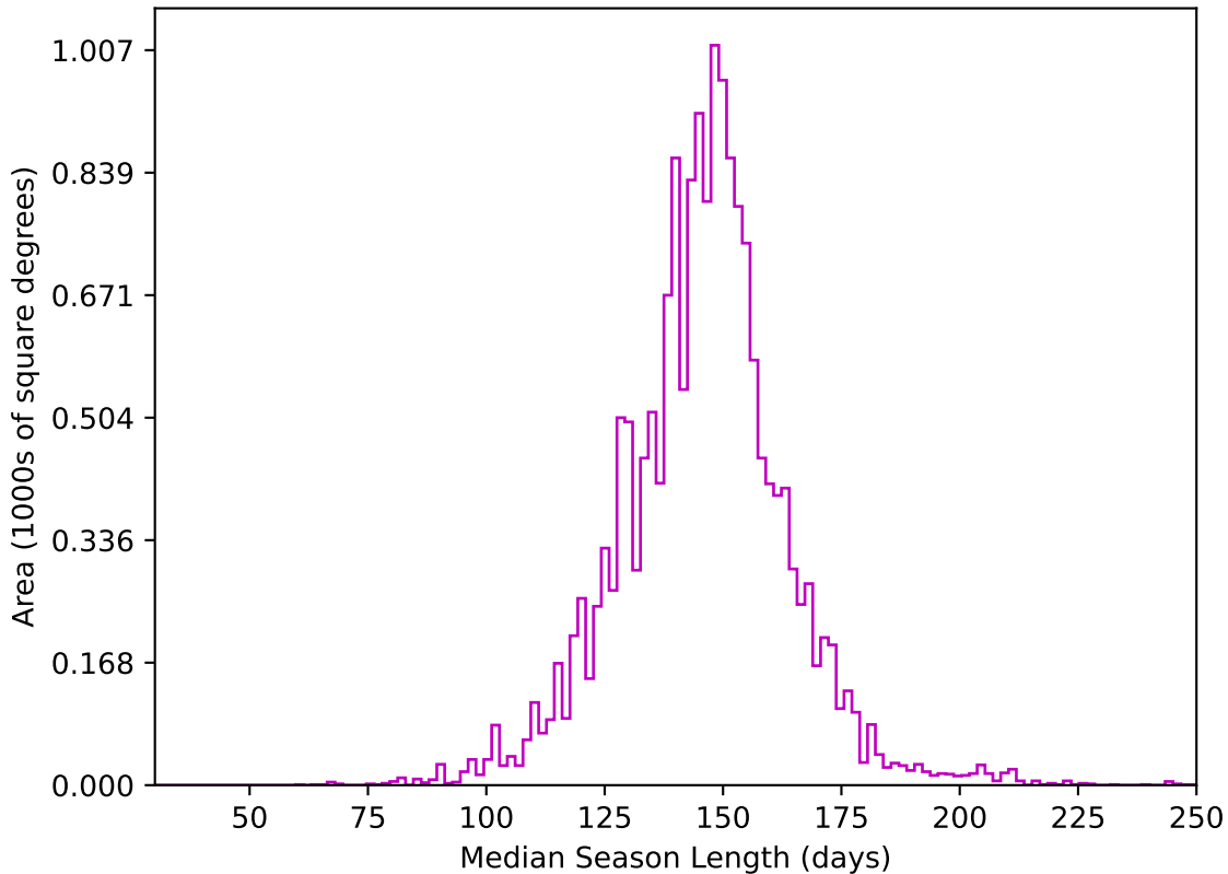
too_elab_r64_d3_ugrizy_v3.4_10yrs WFD z band: Median Season Length
