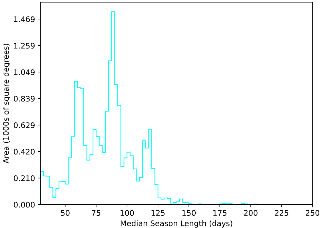
too_elab_r64_d3_ugrizy_v3.4_10yrs WFD u band: Median Season Length
