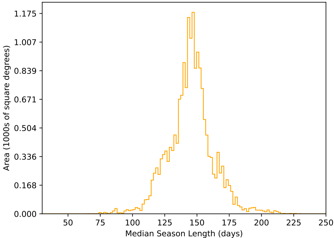
too_elab_r64_d3_ugrizy_v3.4_10yrs WFD r band: Median Season Length
