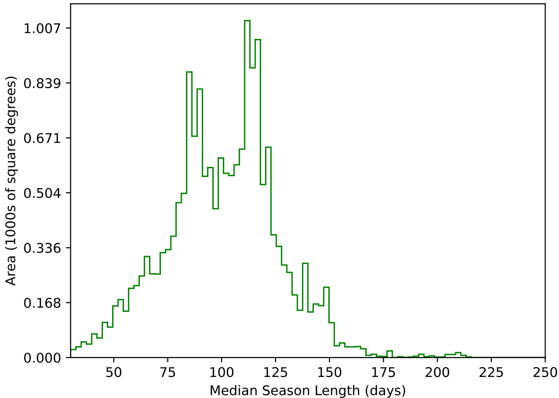
too_elab_r64_d3_ugrizy_v3.4_10yrs WFD g band: Median Season Length
