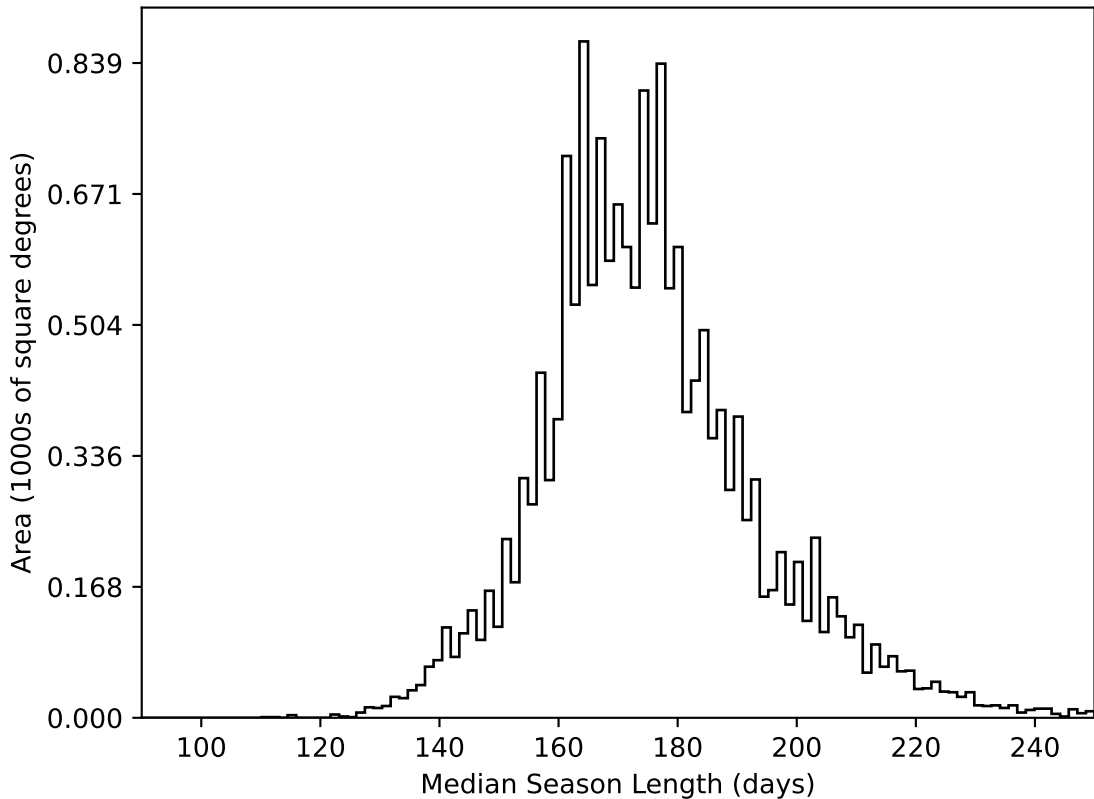
too_elab_r64_d3_ugrizy_v3.4_10yrs WFD all bands: Median Season Length
