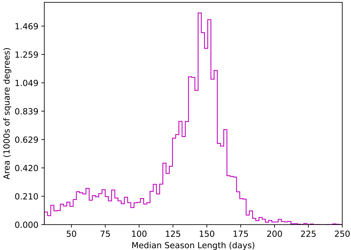
too_elab_r64_d3_ugrizy_v3.4_10yrs All sky z band: Median Season Length
