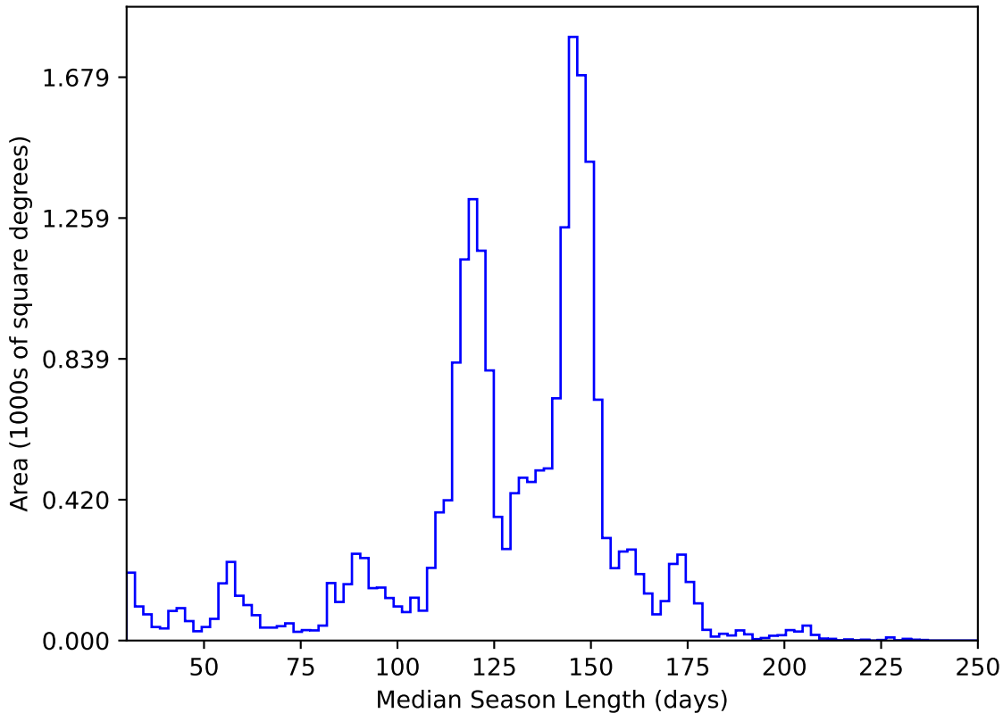
too_elab_r64_d3_ugrizy_v3.4_10yrs All sky y band: Median Season Length
