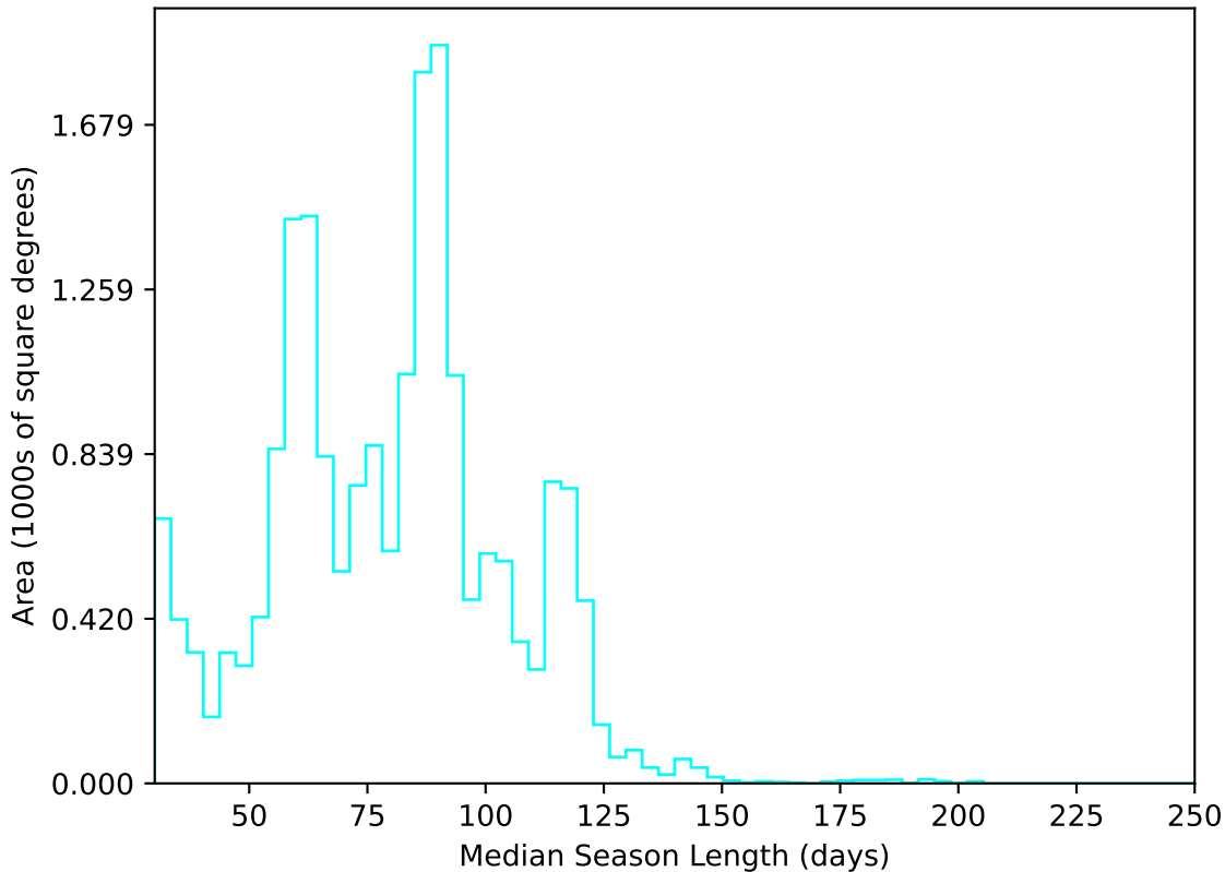
too_elab_r64_d3_ugrizy_v3.4_10yrs All sky u band: Median Season Length
