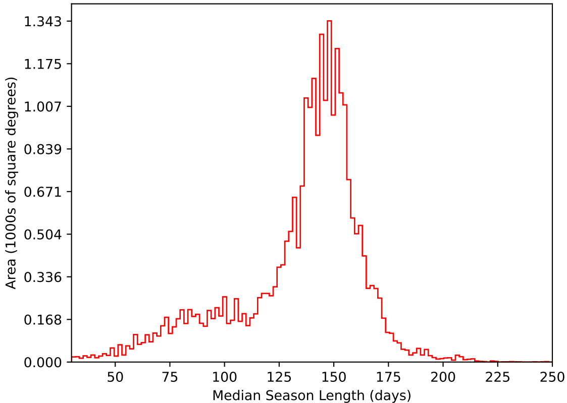
too_elab_r64_d3_ugrizy_v3.4_10yrs All sky i band: Median Season Length
