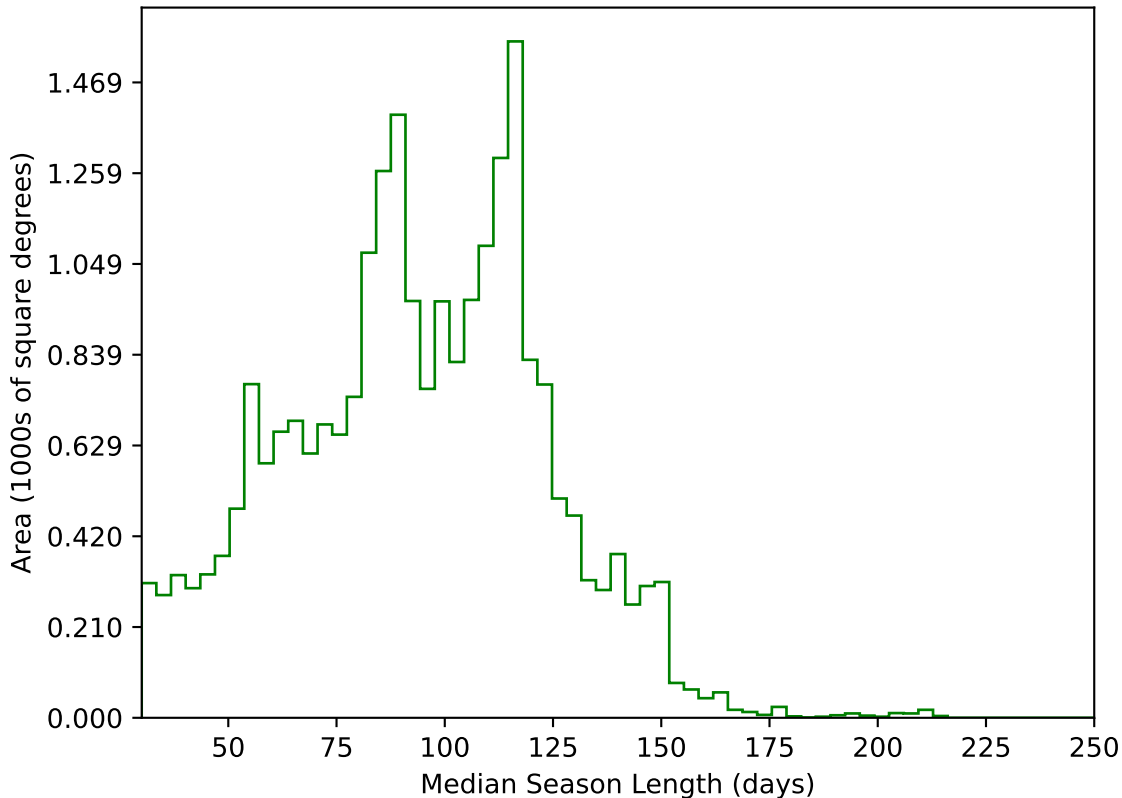
too_elab_r64_d3_ugrizy_v3.4_10yrs All sky g band: Median Season Length
