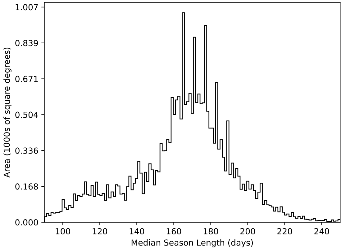
too_elab_r64_d3_ugrizy_v3.4_10yrs All sky all bands: Median Season Length
