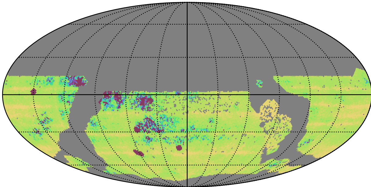
too_elab_r64_d3_ugrizy_v3.4_10yrs WFD: Median Intra-Night Gap
