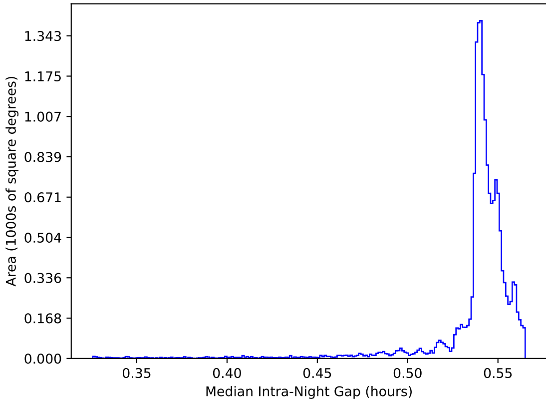
too_elab_r64_d3_ugrizy_v3.4_10yrs WFD: Median Intra-Night Gap
