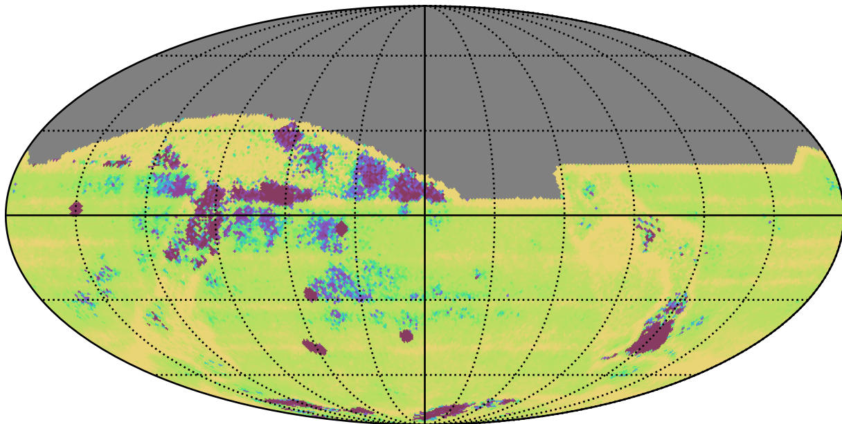
too_elab_r64_d3_ugrizy_v3.4_10yrs All sky: Median Intra-Night Gap
