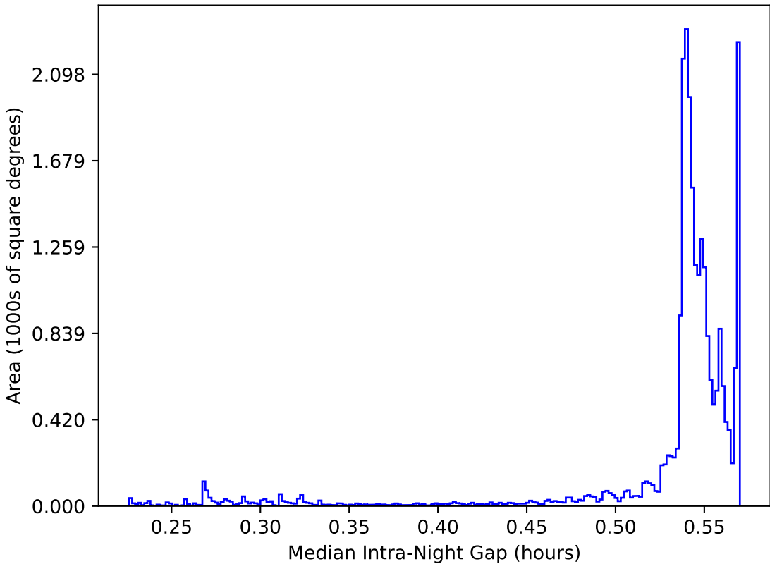
too_elab_r64_d3_ugrizy_v3.4_10yrs All sky: Median Intra-Night Gap
