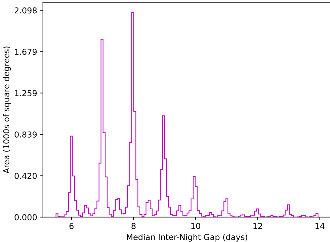
too_elab_r64_d3_ugrizy_v3.4_10yrs WFD z band: Median Inter-Night Gap
