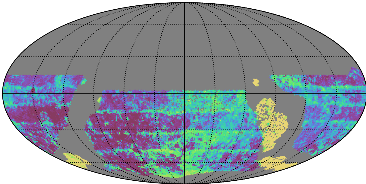
too_elab_r64_d3_ugrizy_v3.4_10yrs WFD y band: Median Inter-Night Gap
