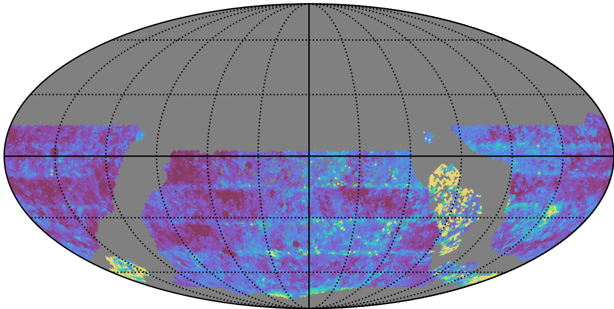
too_elab_r64_d3_ugrizy_v3.4_10yrs WFD u band: Median Inter-Night Gap
