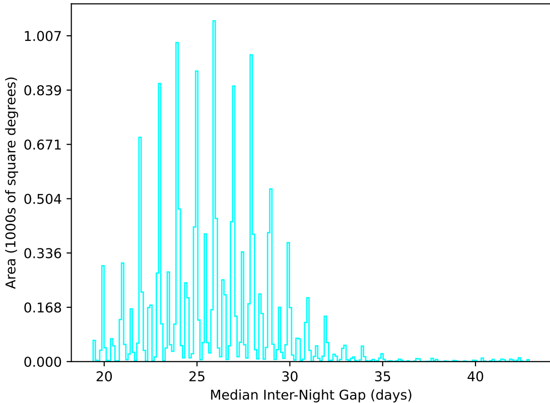
too_elab_r64_d3_ugrizy_v3.4_10yrs WFD u band: Median Inter-Night Gap
