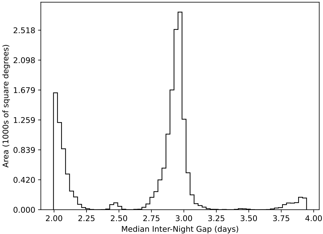
too_elab_r64_d3_ugrizy_v3.4_10yrs WFD all bands: Median Inter-Night Gap
