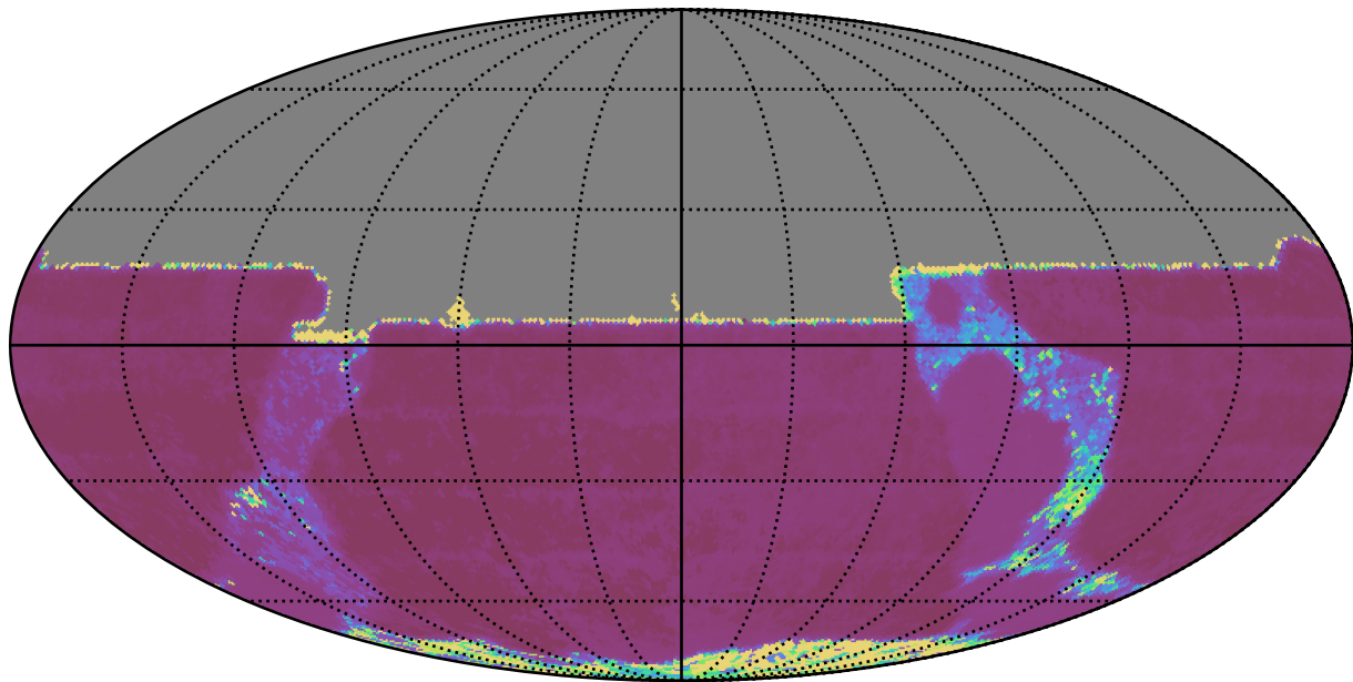
too_elab_r64_d3_ugrizy_v3.4_10yrs All sky y band: Median Inter-Night Gap
