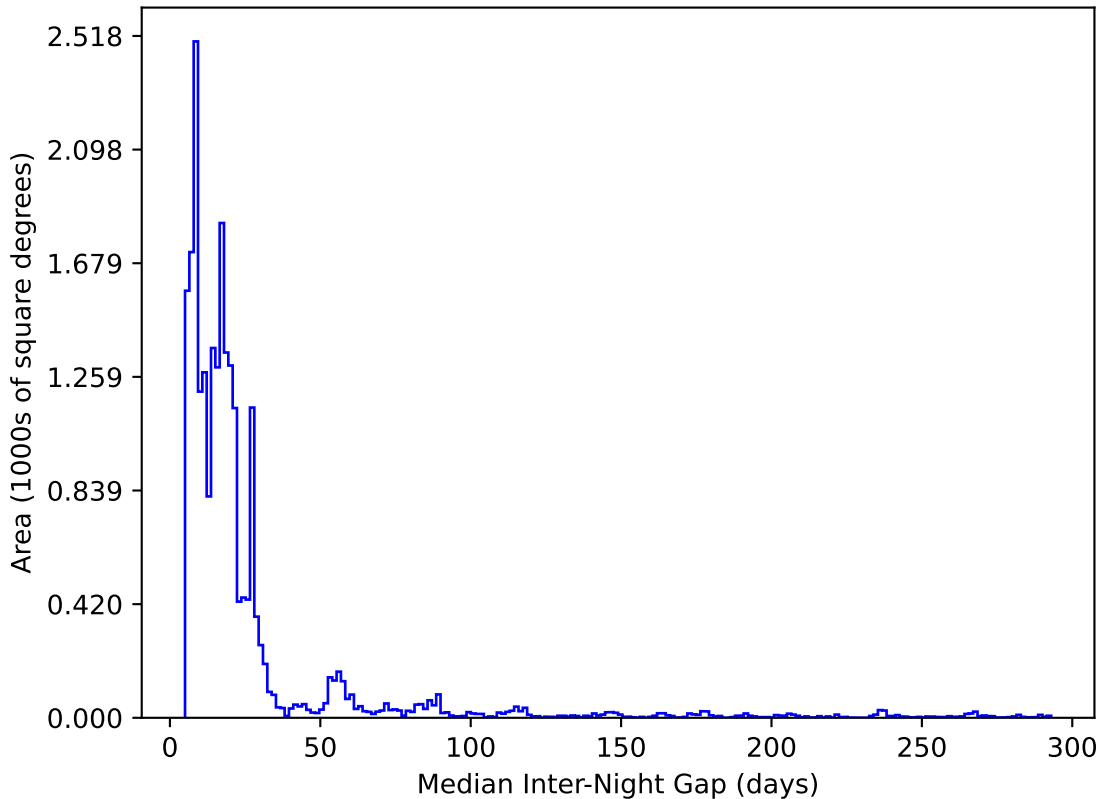
too_elab_r64_d3_ugrizy_v3.4_10yrs All sky y band: Median Inter-Night Gap
