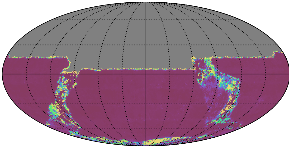
too_elab_r64_d3_ugrizy_v3.4_10yrs All sky u band: Median Inter-Night Gap
