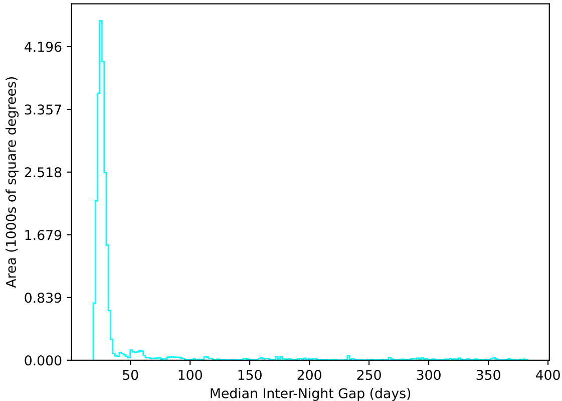
too_elab_r64_d3_ugrizy_v3.4_10yrs All sky u band: Median Inter-Night Gap
