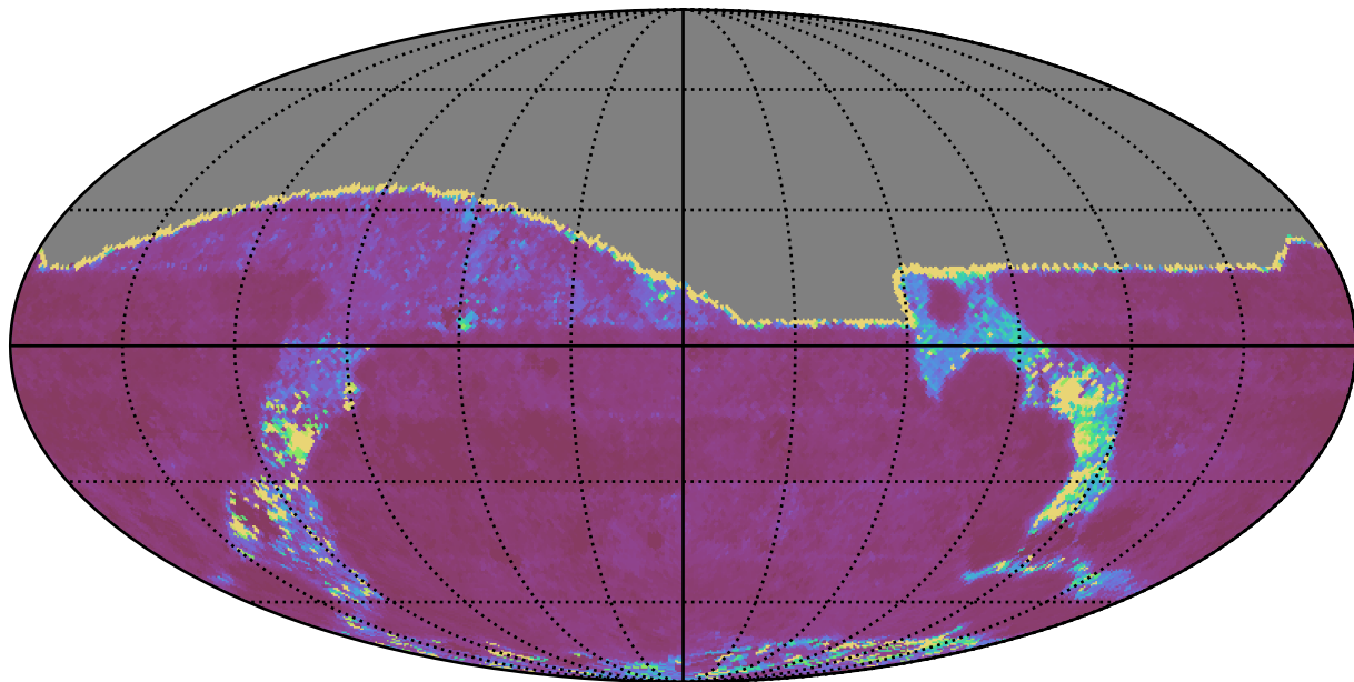
too_elab_r64_d3_ugrizy_v3.4_10yrs All sky g band: Median Inter-Night Gap
