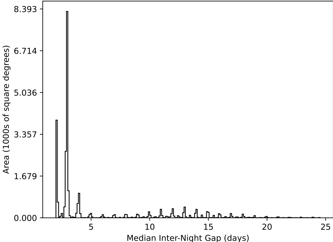
too_elab_r64_d3_ugrizy_v3.4_10yrs All sky all bands: Median Inter-Night Gap
