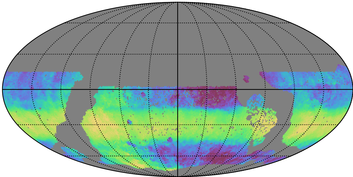
too_elab_r64_d3_ugrizy_v3.4_10yrs WFD y band: Median HA
