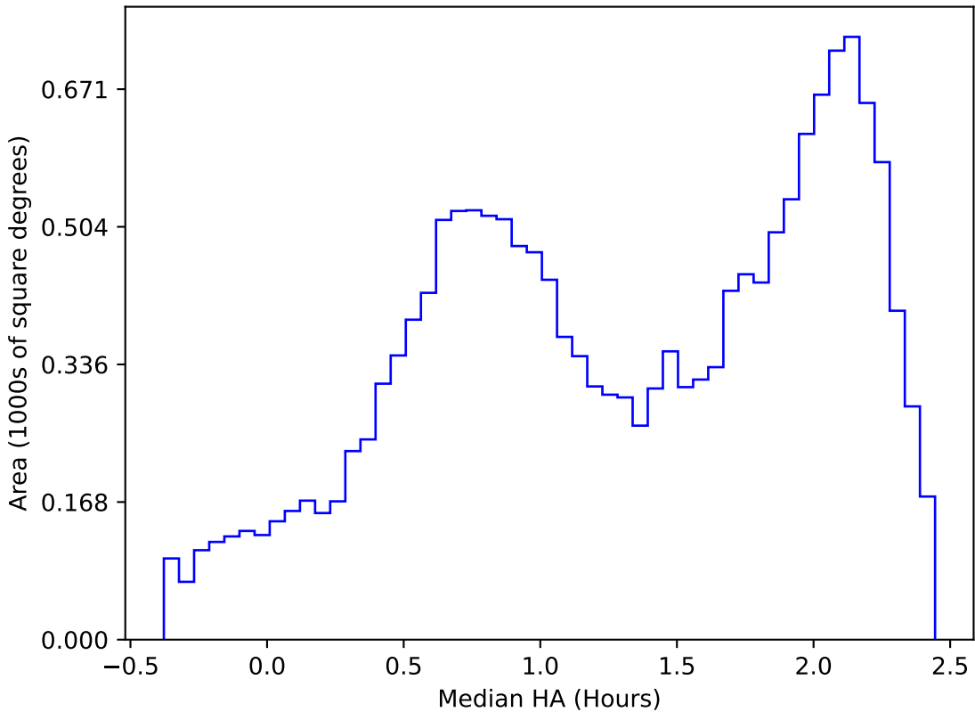
too_elab_r64_d3_ugrizy_v3.4_10yrs WFD y band: Median HA
