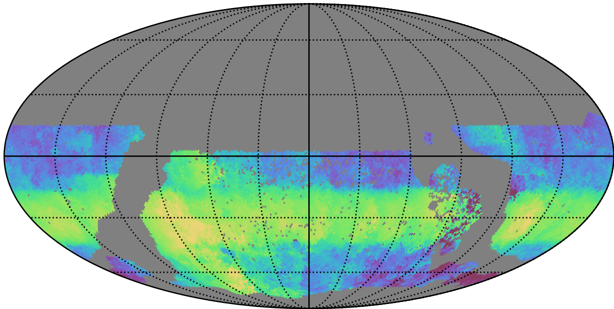
too_elab_r64_d3_ugrizy_v3.4_10yrs WFD u band: Median HA
