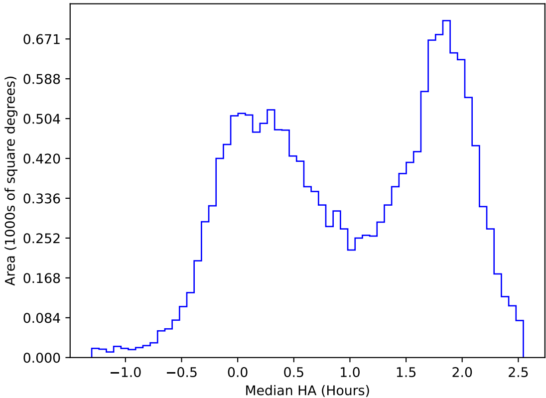
too_elab_r64_d3_ugrizy_v3.4_10yrs WFD u band: Median HA
