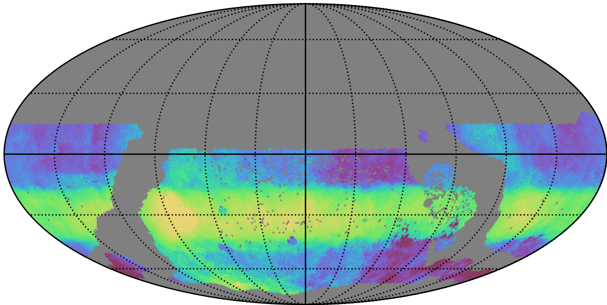
too_elab_r64_d3_ugrizy_v3.4_10yrs WFD r band: Median HA
