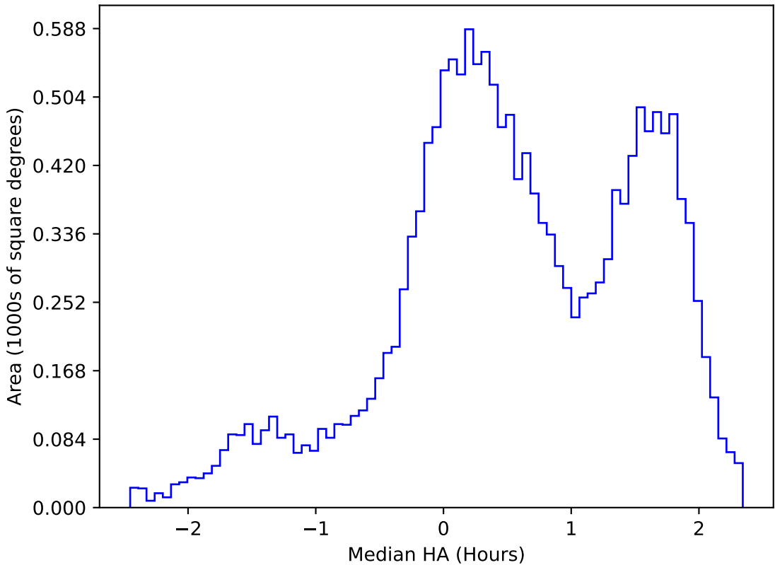
too_elab_r64_d3_ugrizy_v3.4_10yrs WFD g band: Median HA
