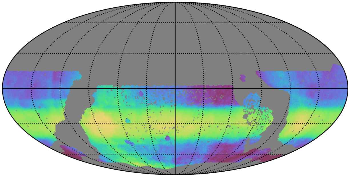
too_elab_r64_d3_ugrizy_v3.4_10yrs WFD all bands: Median HA
