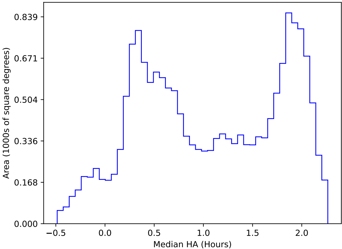
too_elab_r64_d3_ugrizy_v3.4_10yrs WFD all bands: Median HA
